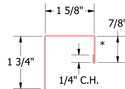
J Channel
