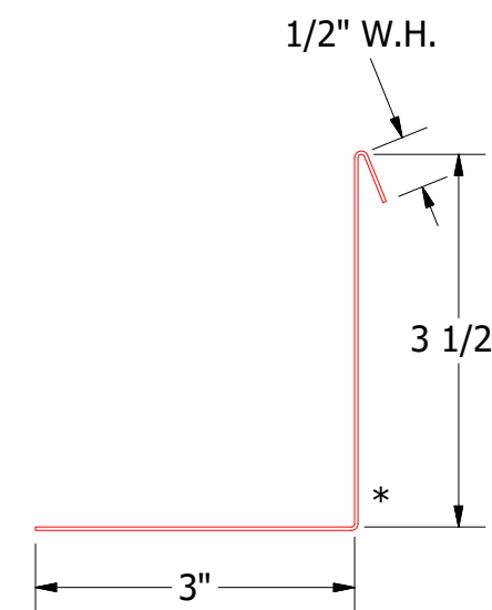
Angle Trim with Return
