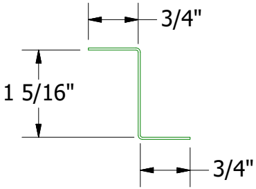
Support Z
