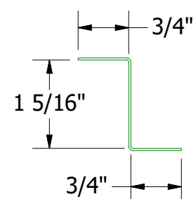
Support Z
