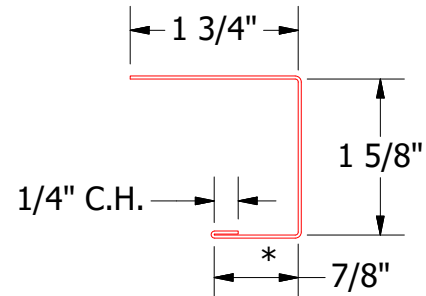
J Channel
