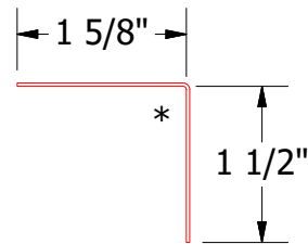
Angle Trim
