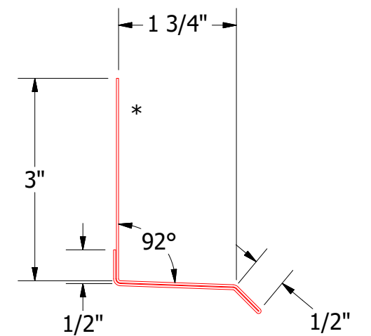
Base Trim
