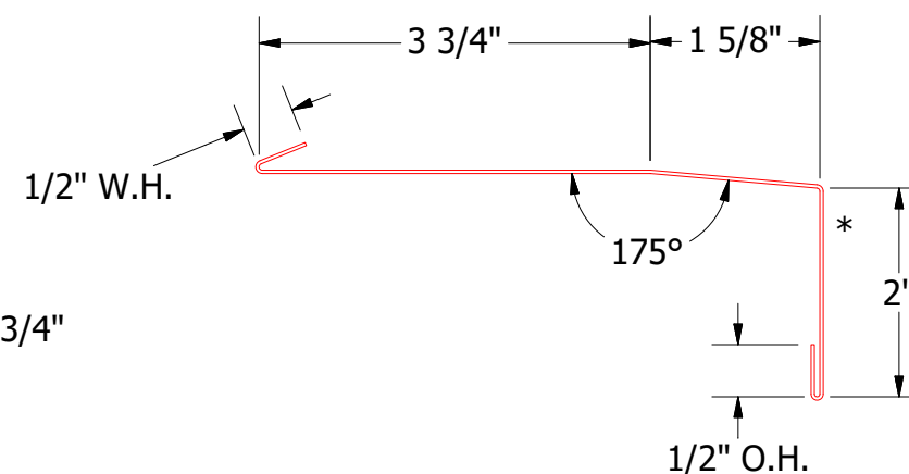
Window Sill Trim
