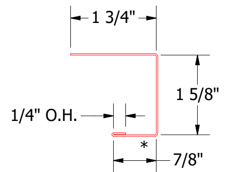
J Channel
