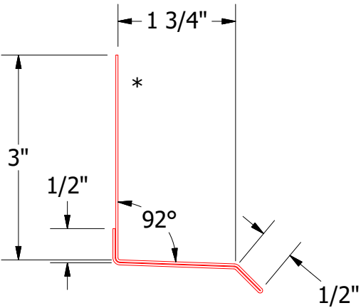
Base Trim - Standard
