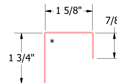
J Closure
