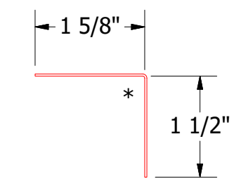
Angle Trim
