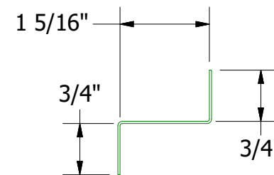
Support Z
