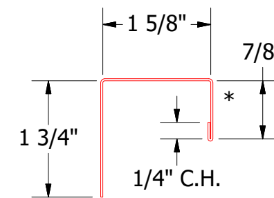
J Channel
