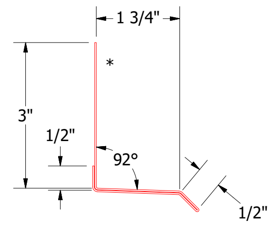
Base Trim - Standard
