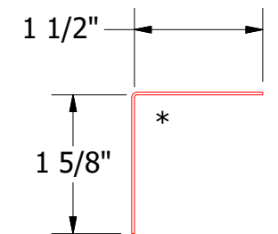
Angle Trim
