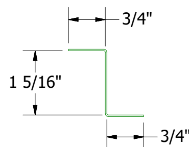
Support Z
