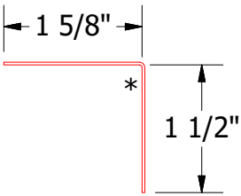
Angle Trim
