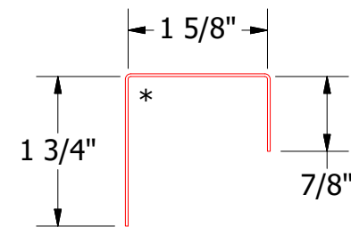
J Closure
