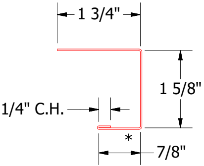
J Channel
