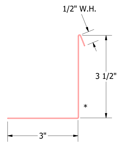
Angle Trim with Return
