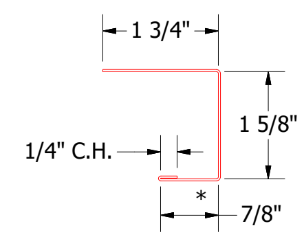
J Channel
