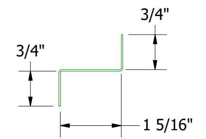
Support Z
