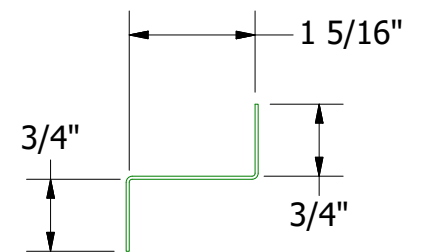
Support Z
