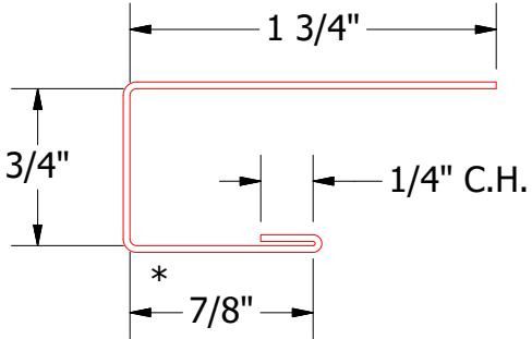
OPA034 - J Channel
