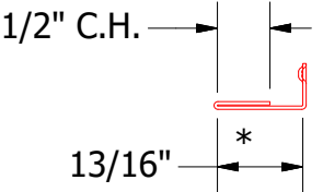
UNS078 - Snap J Cover
