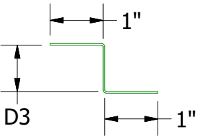
Support Z DWA681: D3 = 1" DSA681: D3 = 1 5/8"
