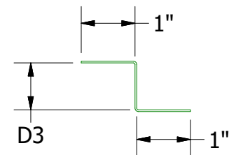
Support Z DWA681: D3 = 1" DSA681: D3 = 1 5/8"
