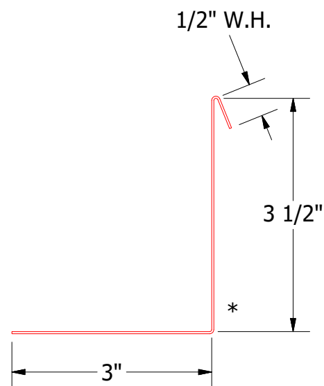
DWA683/DSA683 - Angle Trim With Return
