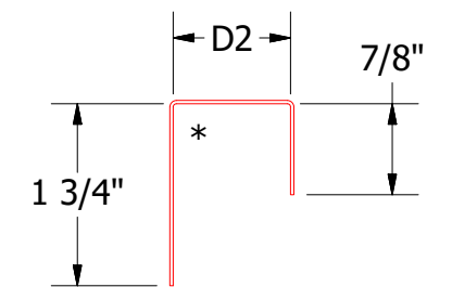
J Closure DWA270: D2 = 1 1/8" DSA270: D2 = 1 7/8"
