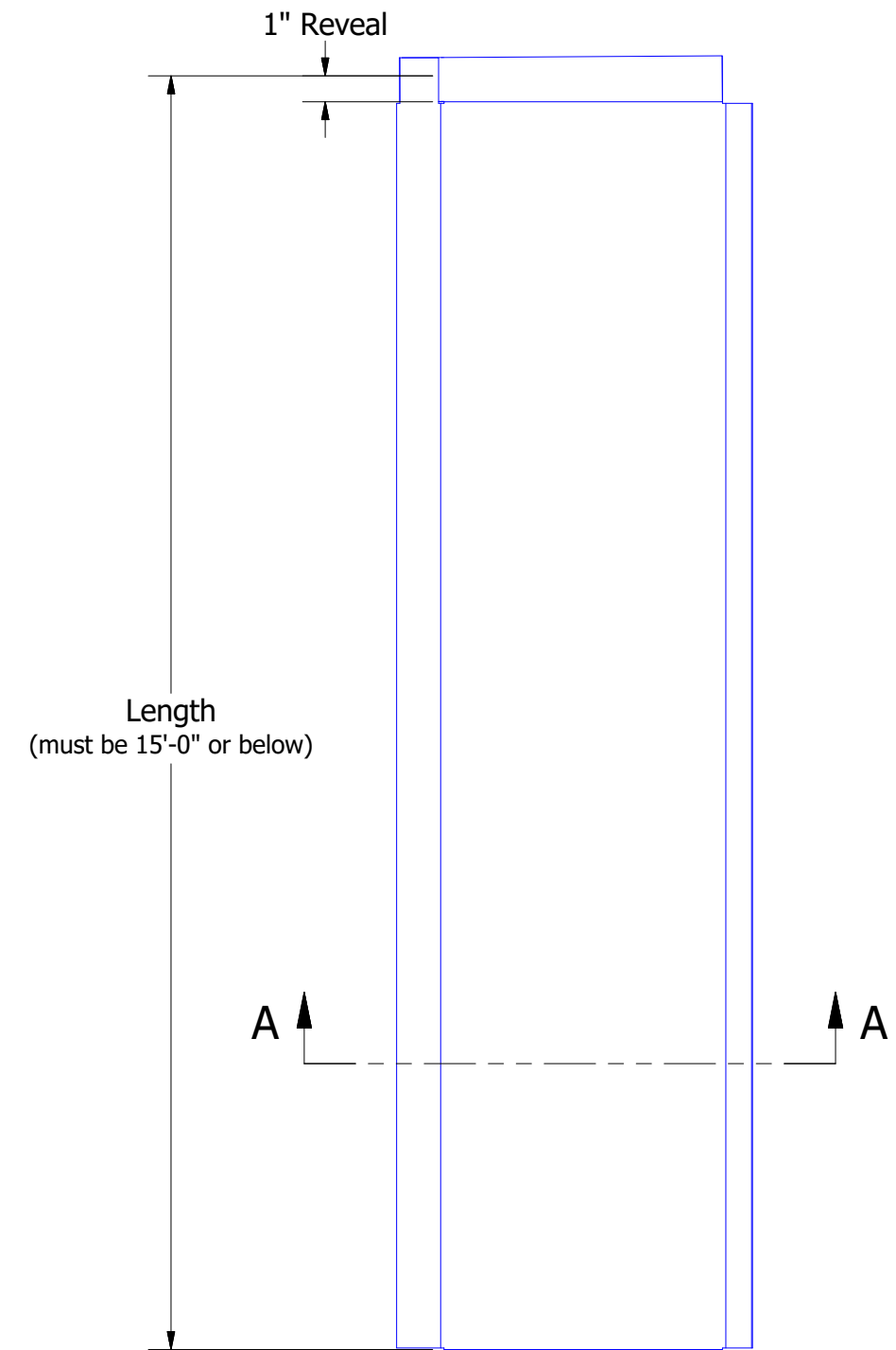
Vertical Panel
