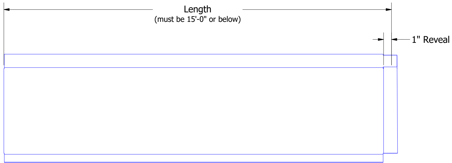
Horizontal Panel
