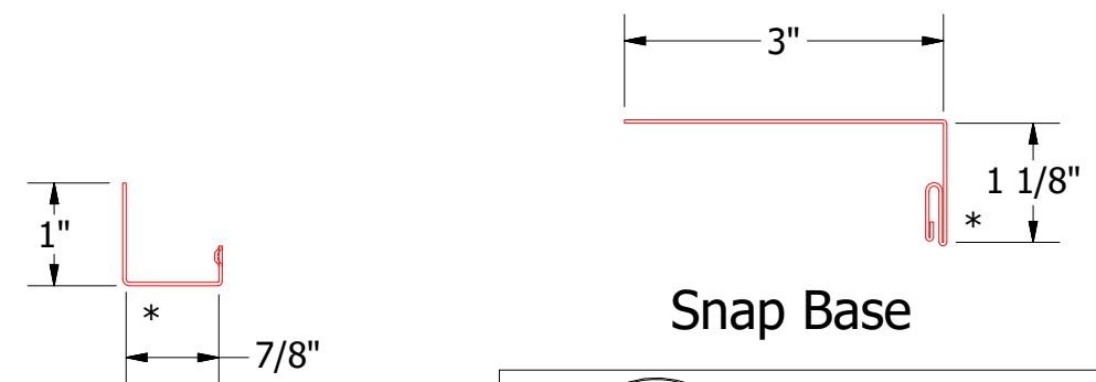
Snap Cover
