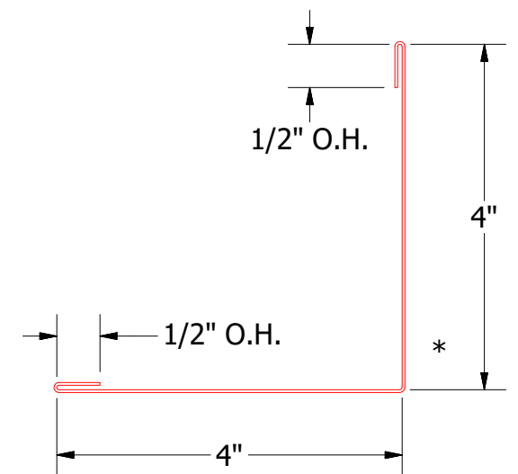
Outside Corner Cap
