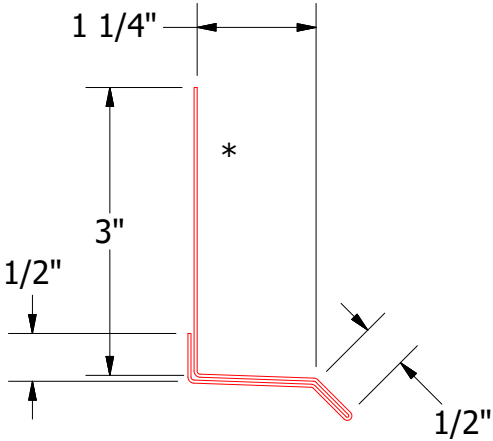
Base Trim
