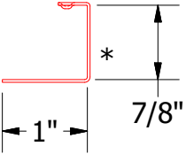
Profiled Snap Cover
