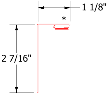
Snap Base
