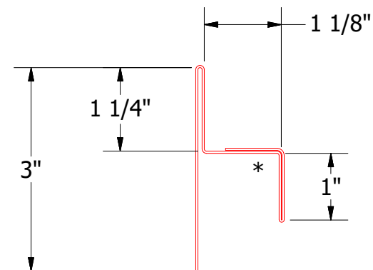
Pocket Z Closure with Return
