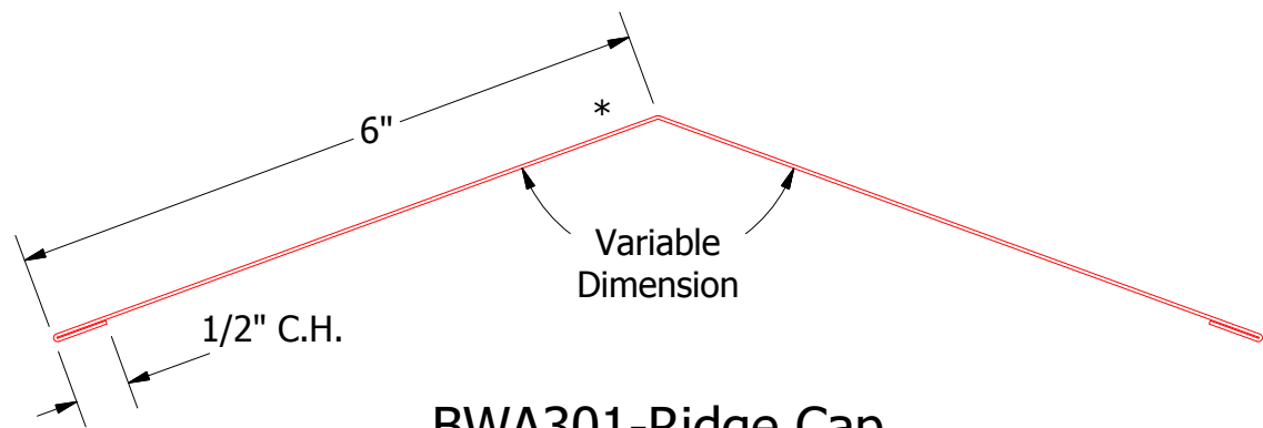
BWA301-Ridge Cap
