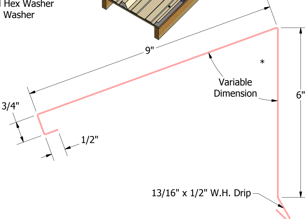
BWA366-Vented Shed Ridge Cap
