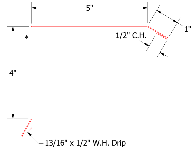
BWA277-Gable Cap - with Angle
