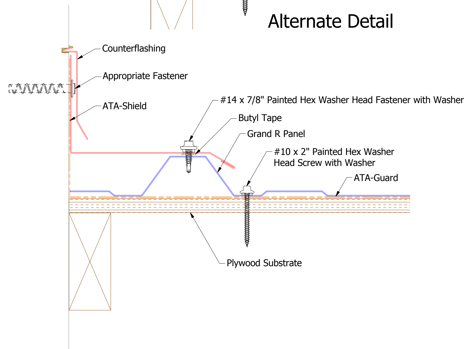
BWA980-Counterflashing
