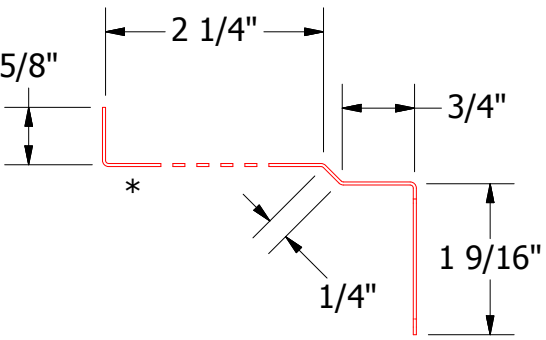
BWA911-Vented Closure Angle
