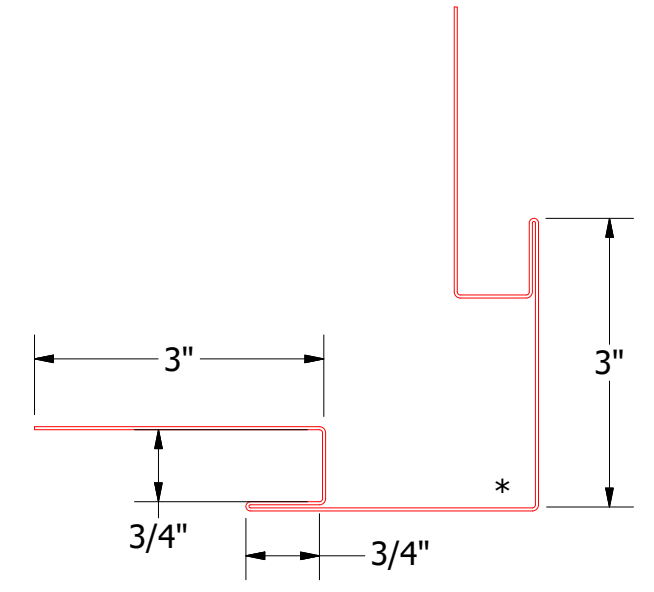
MFA602 - Outside Corner Post
