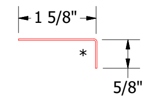
MFA680 - Angle Trim
