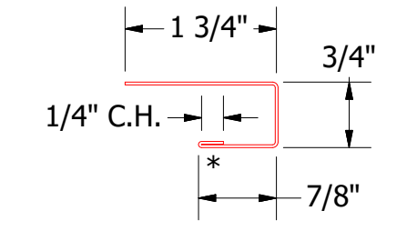
MFA034 - J Channel
