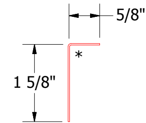
MFA680 - Angle Trim
