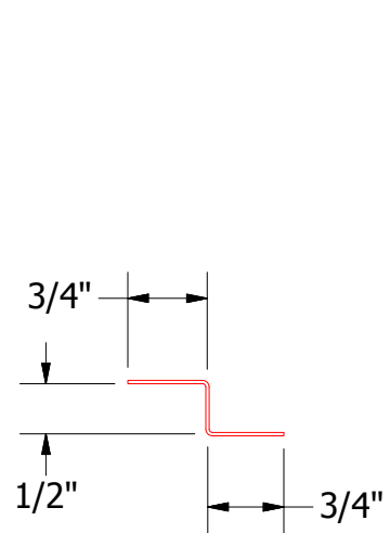
MFA681 - Support Z
