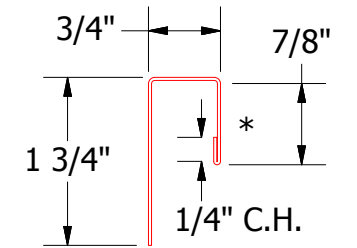
MFA034 - J Channel
