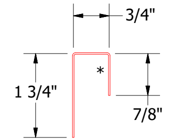
MFA270 - J Closure
