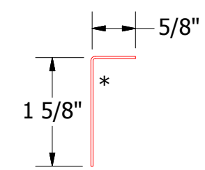
MFA680 - Angle Trim
