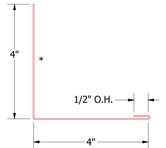
HLA415-Sidewall Channel
