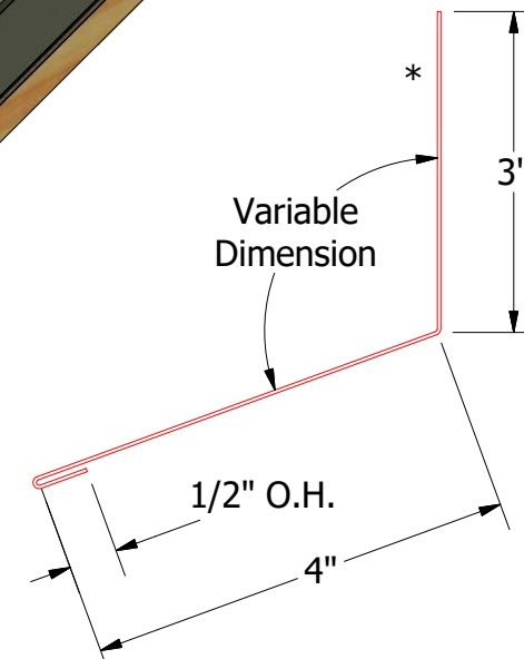
HLA500-Headwall Trim
