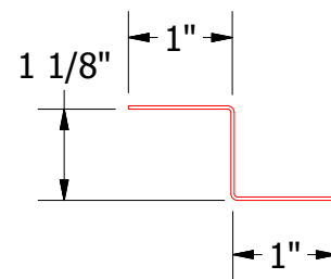
HLA910-Z Closure
