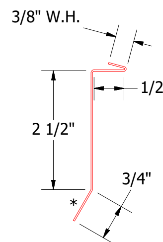
HLA980-Counterflashing
