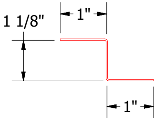
HLA910-Z Closure
